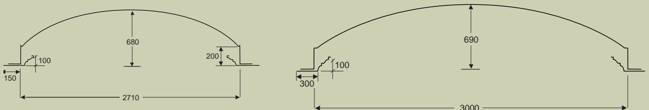
BDM 019 Cross section view
