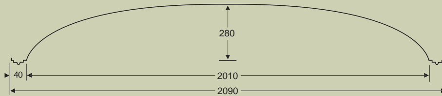
BDM 018 Cross section view
