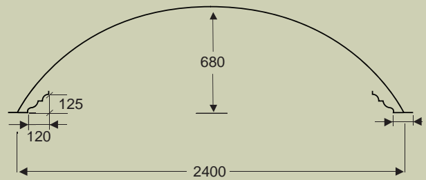
BDM 020 Cross section view
