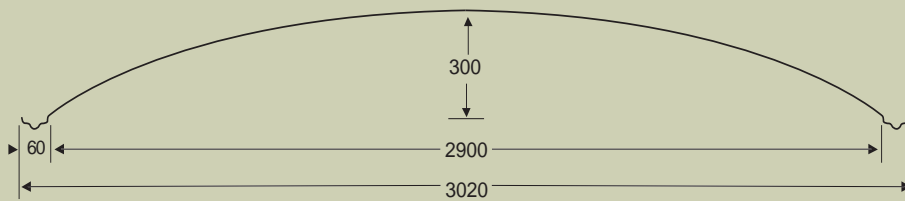
BDM 016 Cross section view
