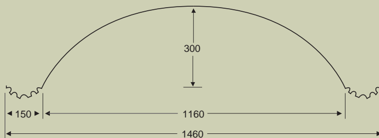
BDM 013 Cross section view
