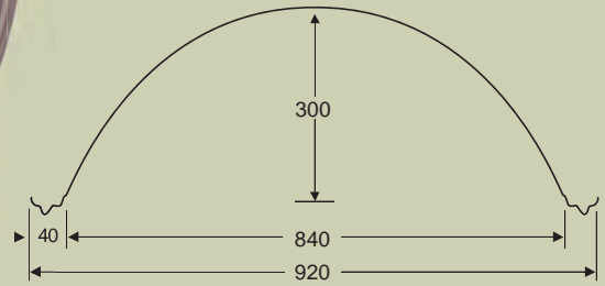
BDM 014 Cross section view
