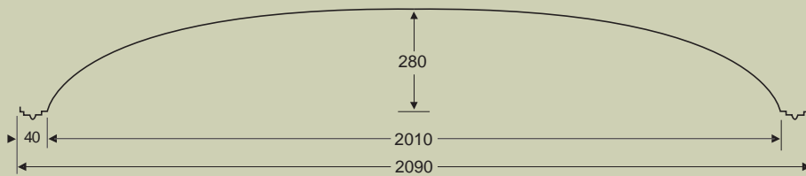
BDM 015 Cross section view
