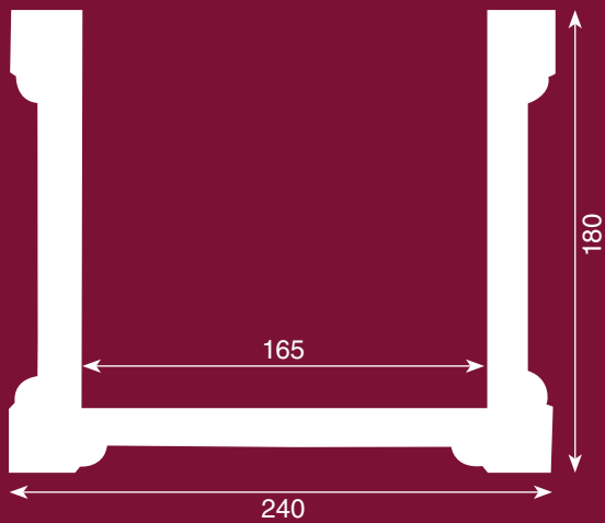
Column Profile
