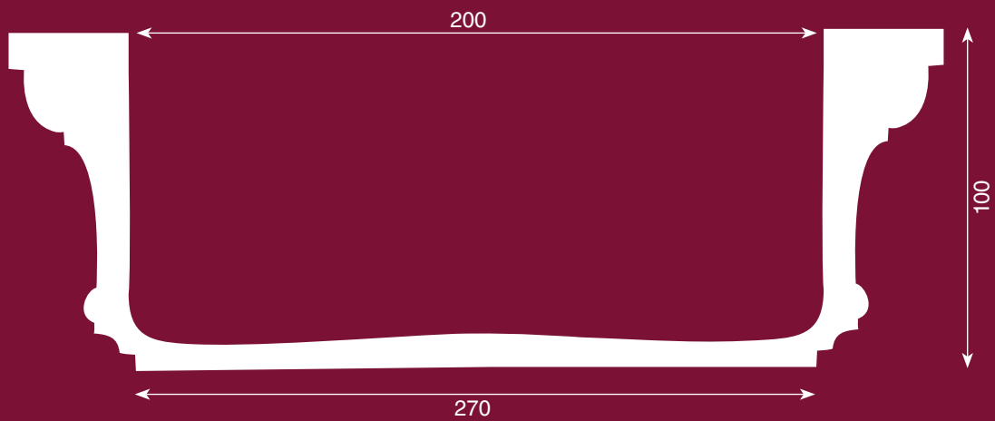
Arch Profile
