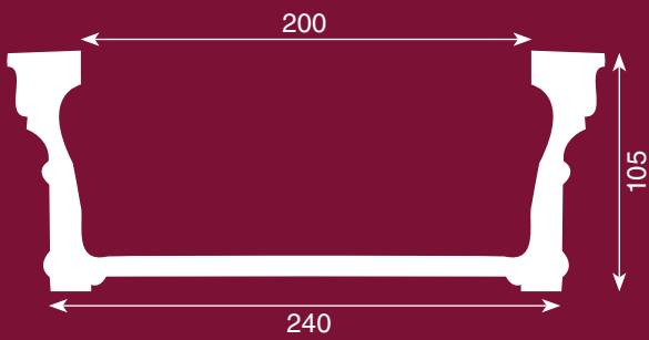
Arch Profile
