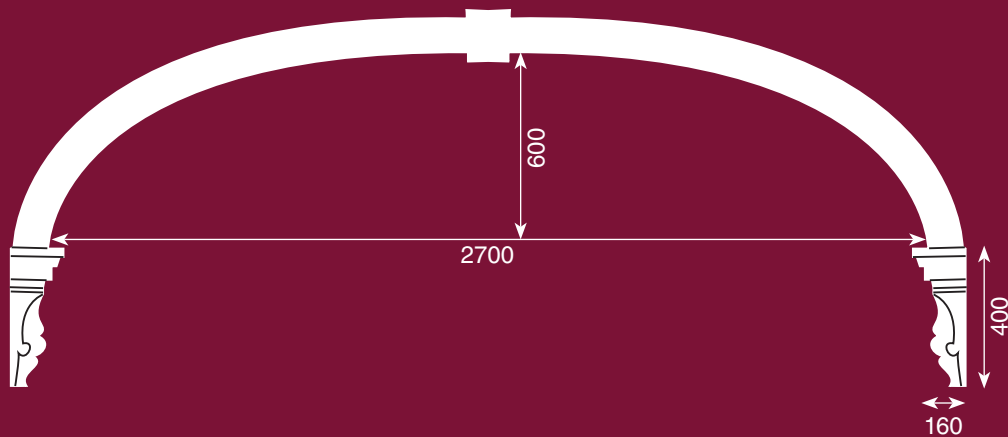
Arch Profile
