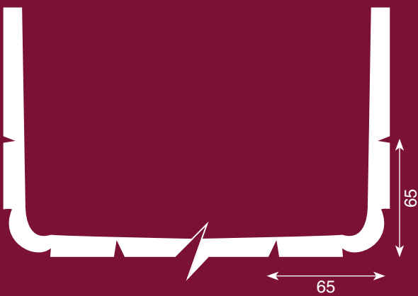
Arch Profile
