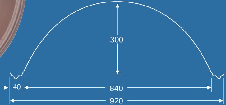
BDM 014 Cross section view
