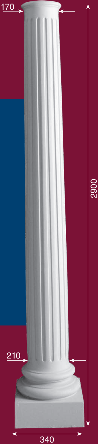
Tapered Column
