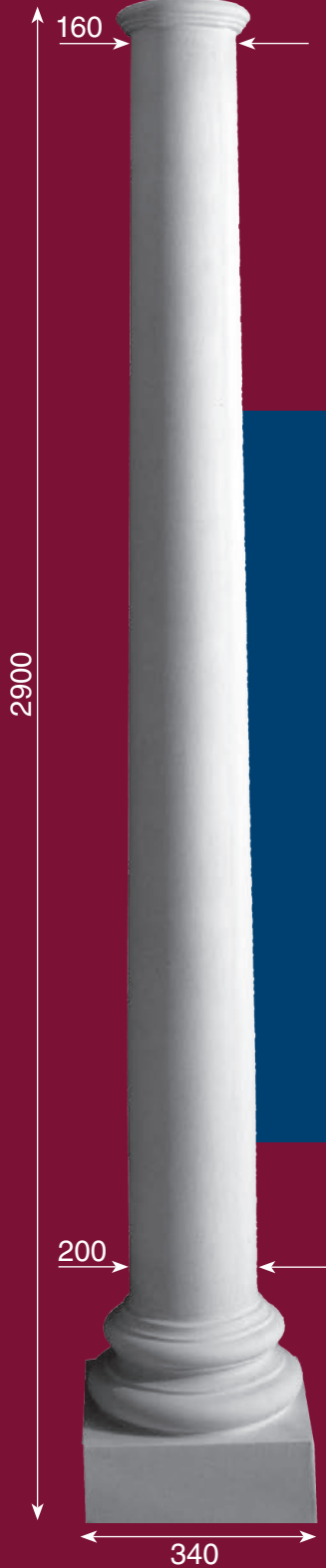
Tapered Column
